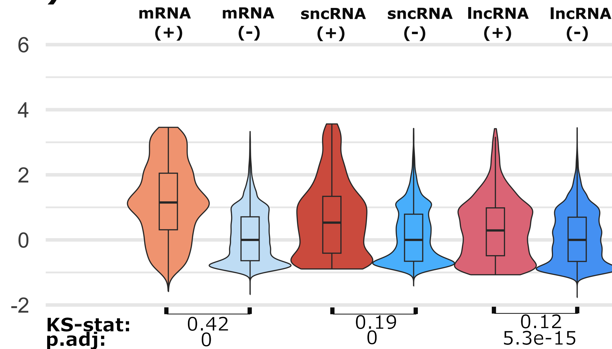
D) GERP-vertebrates
