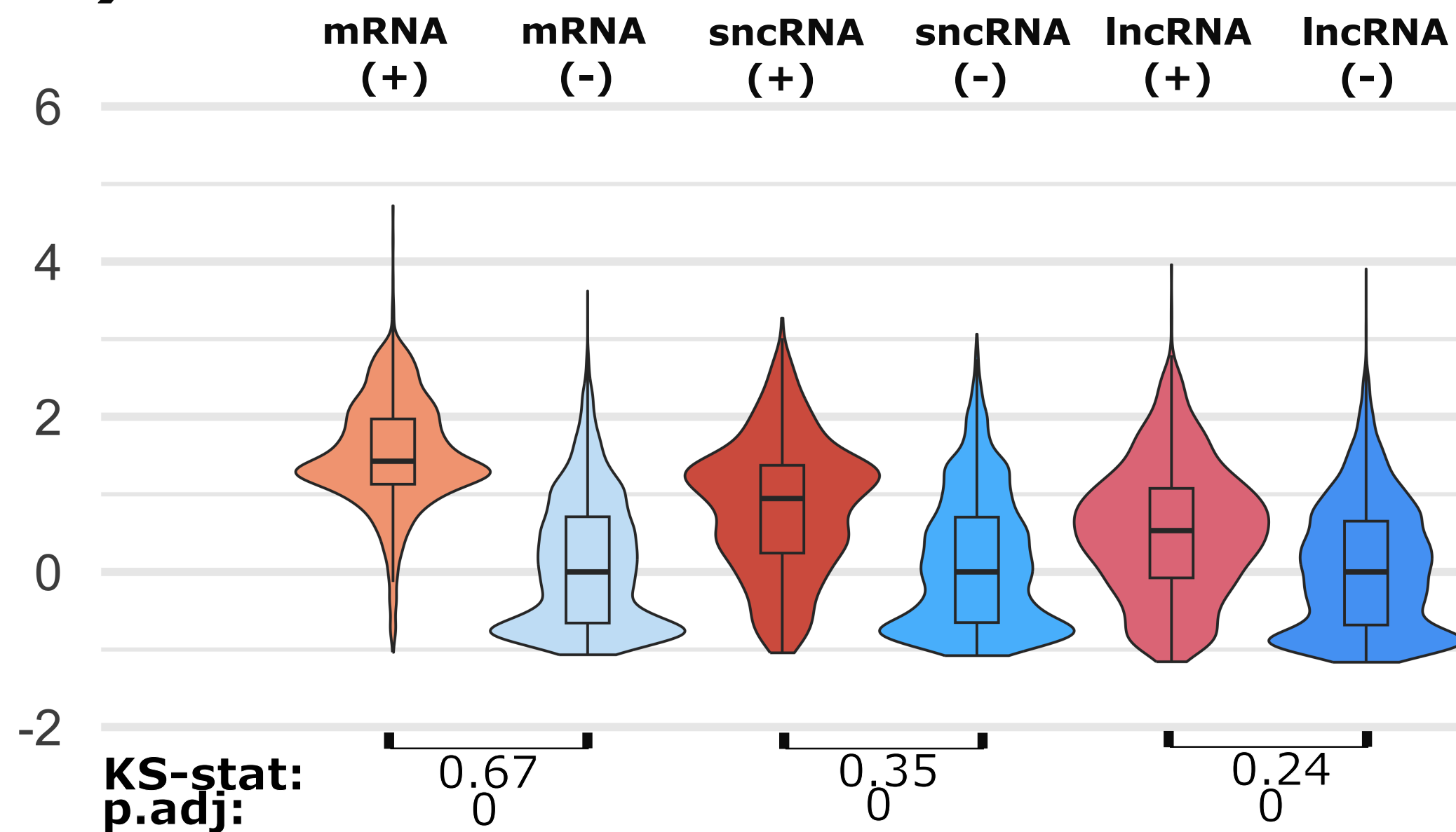
C) GERP-mammals
